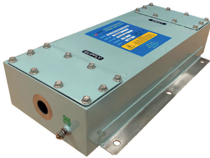
An MPE low-leakage TEMPEST power line filter for naval applications
