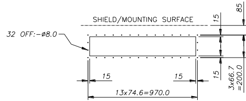
RECOMMENDED CUTOUT DETAIL FOR TERMINATION ENCLOSURES
