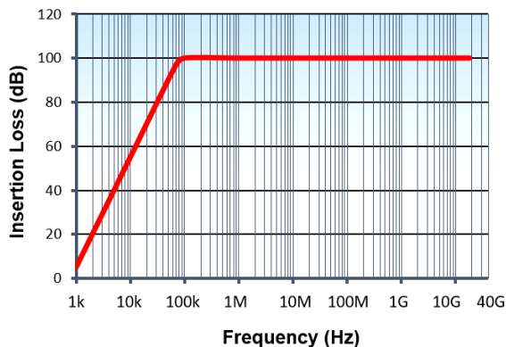
High Current (Low Leakage) Standard Performance 100dB from 100 kHz to 18GHz
